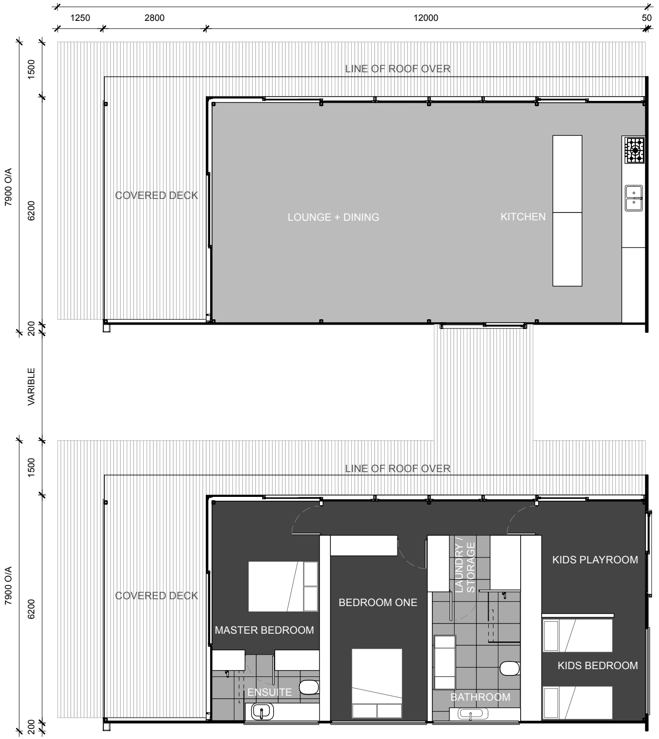
MODULE 110 SPLIT not to scale
