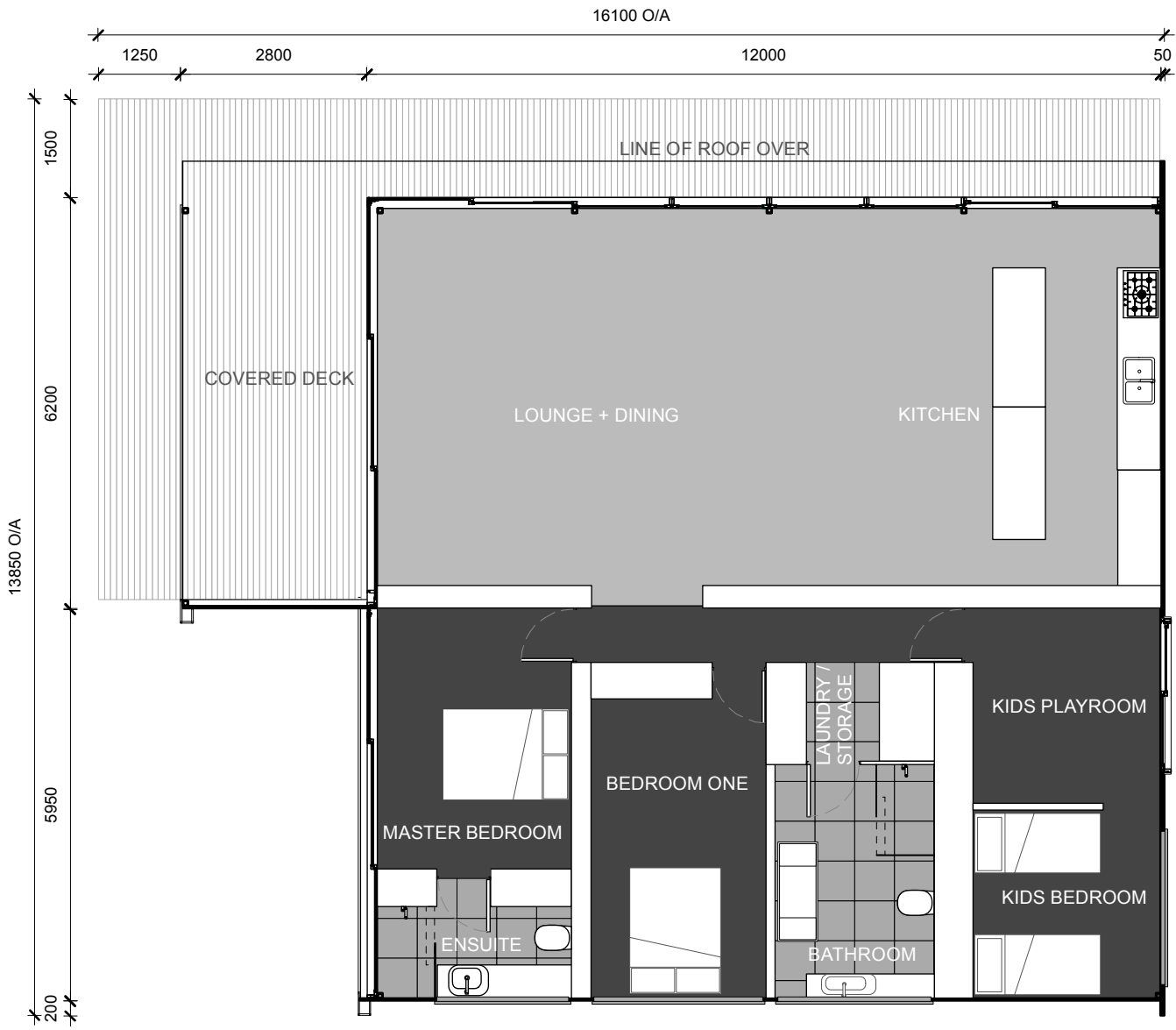
MODULE 110 JOINED not to scale
